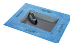
LAUFEN PRO H290031 Mounting box left for Marbond shower trays type DN 40 / height 75 mm, siphon not included
